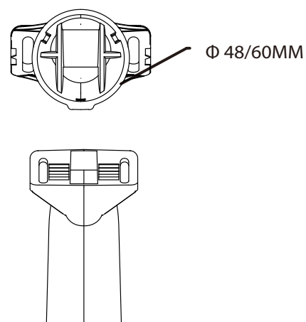
Pole Mount
